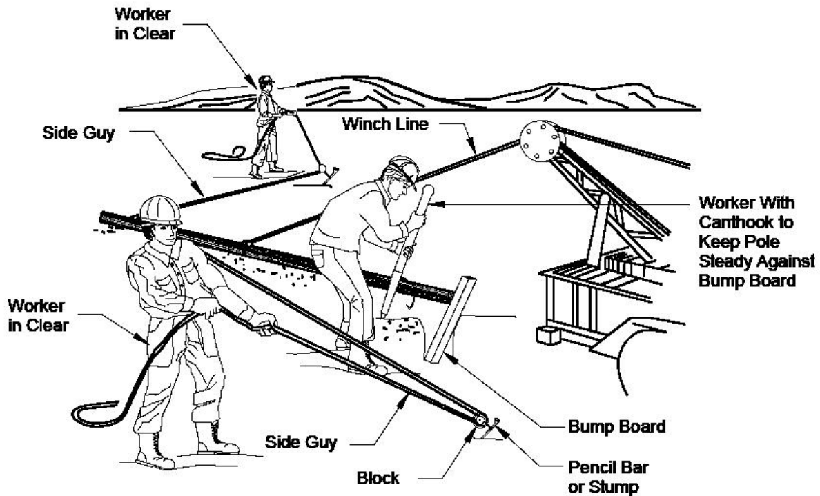
Figure 2 Winch Line Method
