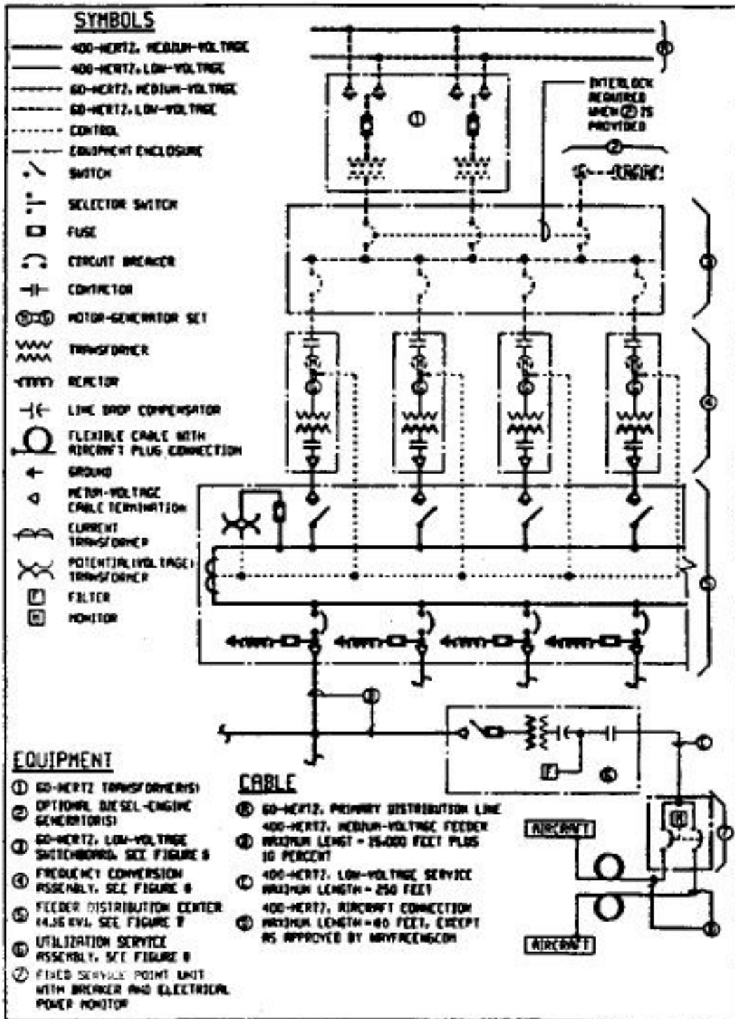
Figure 1a Typical 400 Hz medium voltage system
