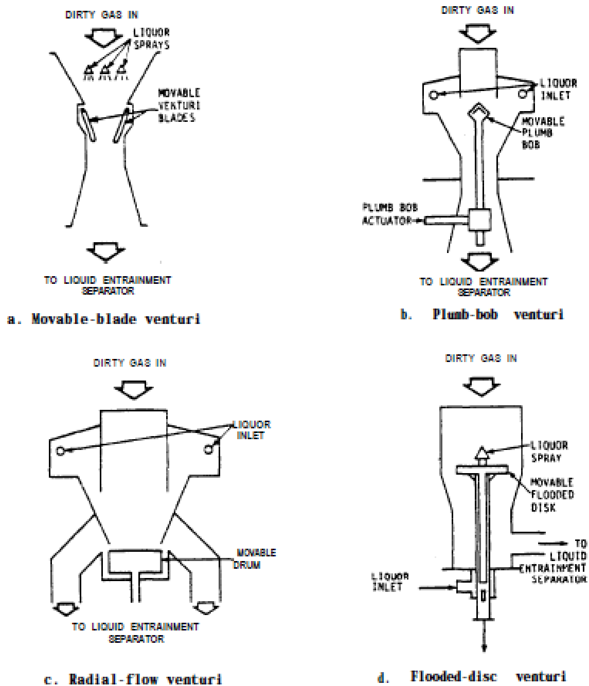
Figure 7-5 Throat sections of variable venturi scrubbers
