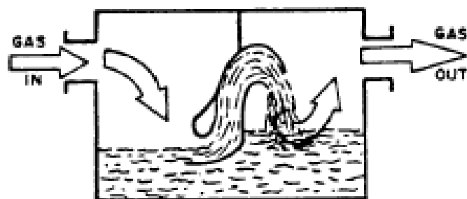
IMPINGEMENT AND ENTRAINMENT SCRUBBER
