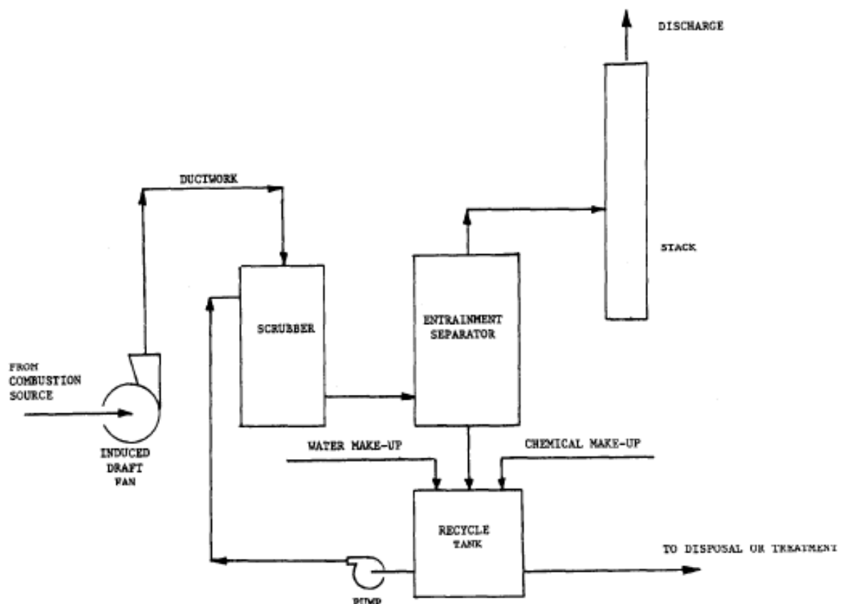
Figure 7-7 Schematic diagram of scrubber flow
