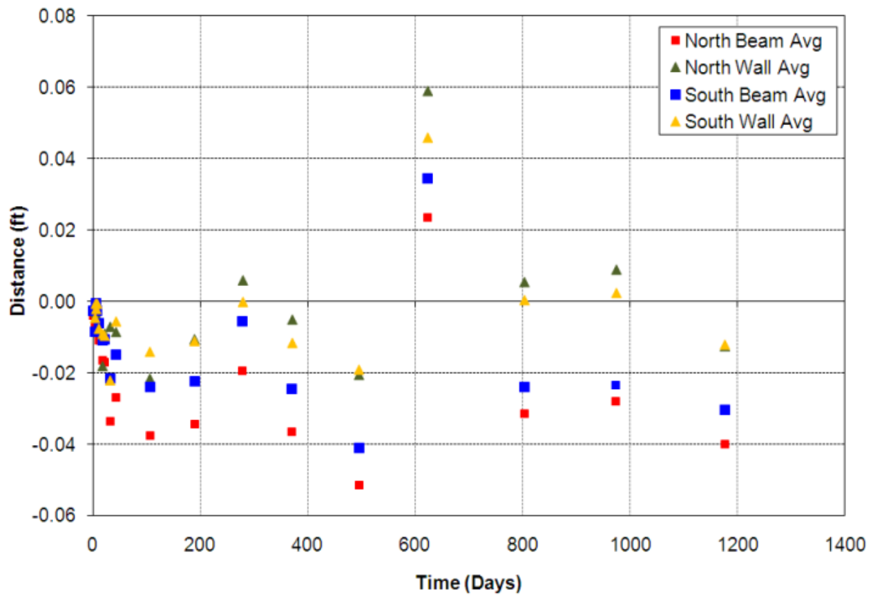
Figure 18. Vine Street GRS-IBS settlement versus time.
