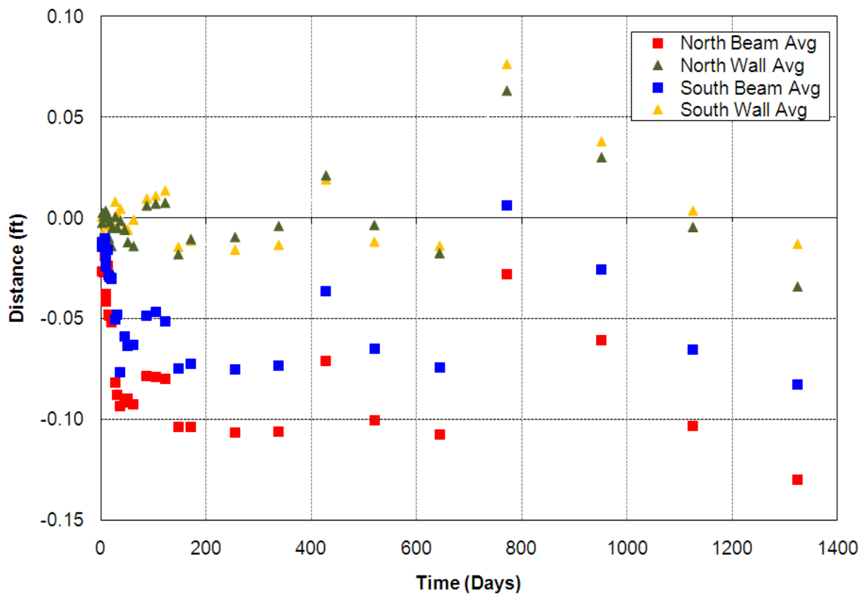
Figure 20. Glenburg Road GRS-IBS settlement versus time.
