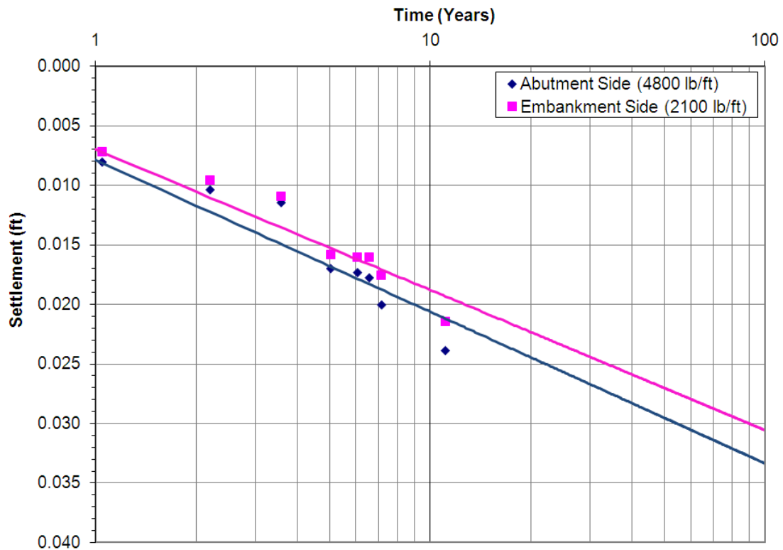
Figure 31. Settlement versus log-time to predict creep settlement for TFHRC tunnel at 100 years.
