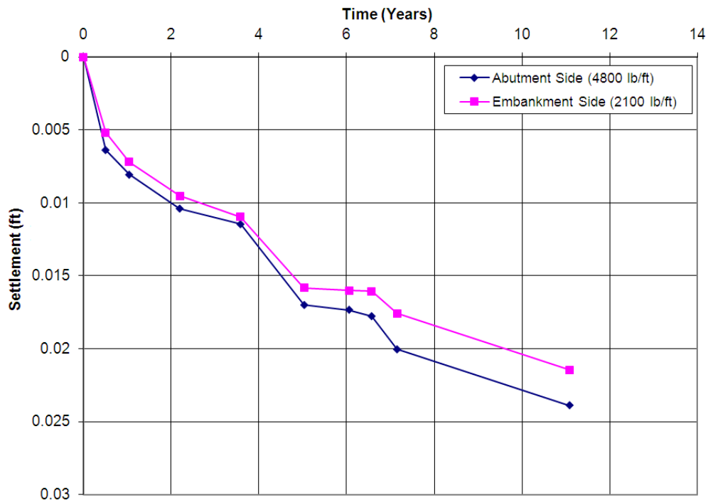
Figure 30. Settlement versus time for TFHRC tunnel.
