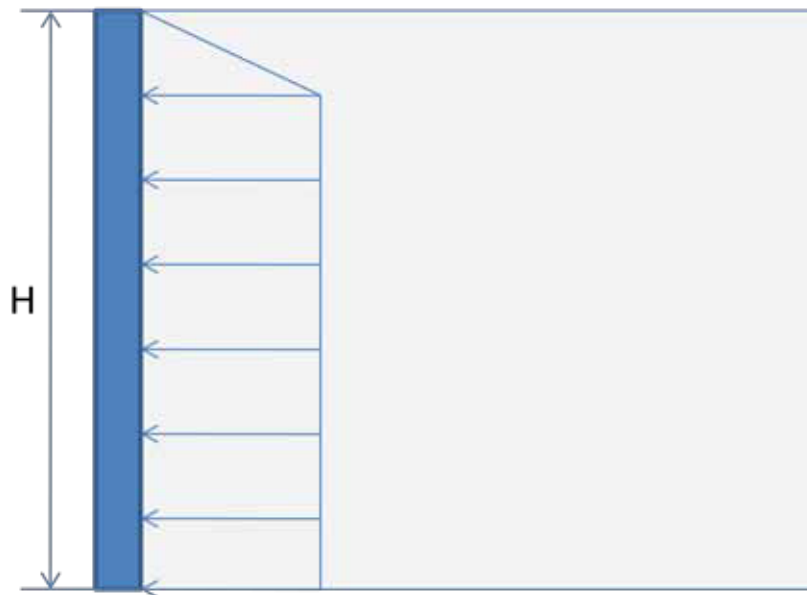
Figure 9. Idealized lateral earth pressure at the face of a GRS structure.
