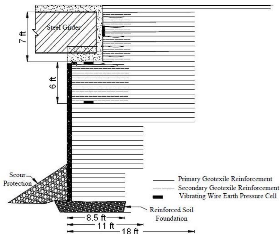
Figure 38. Instrumentation for Tiffin River Bridge.
