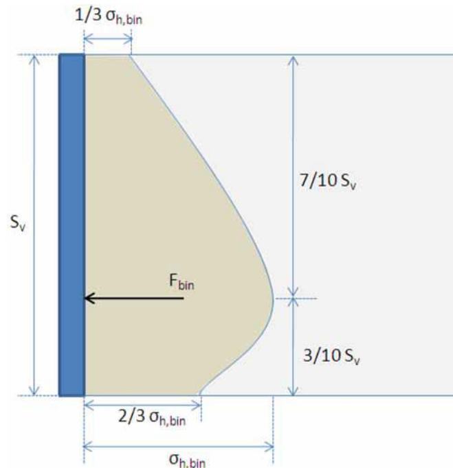
Figure 10. Illustration. Bin pressure diagram for GRS structures.
