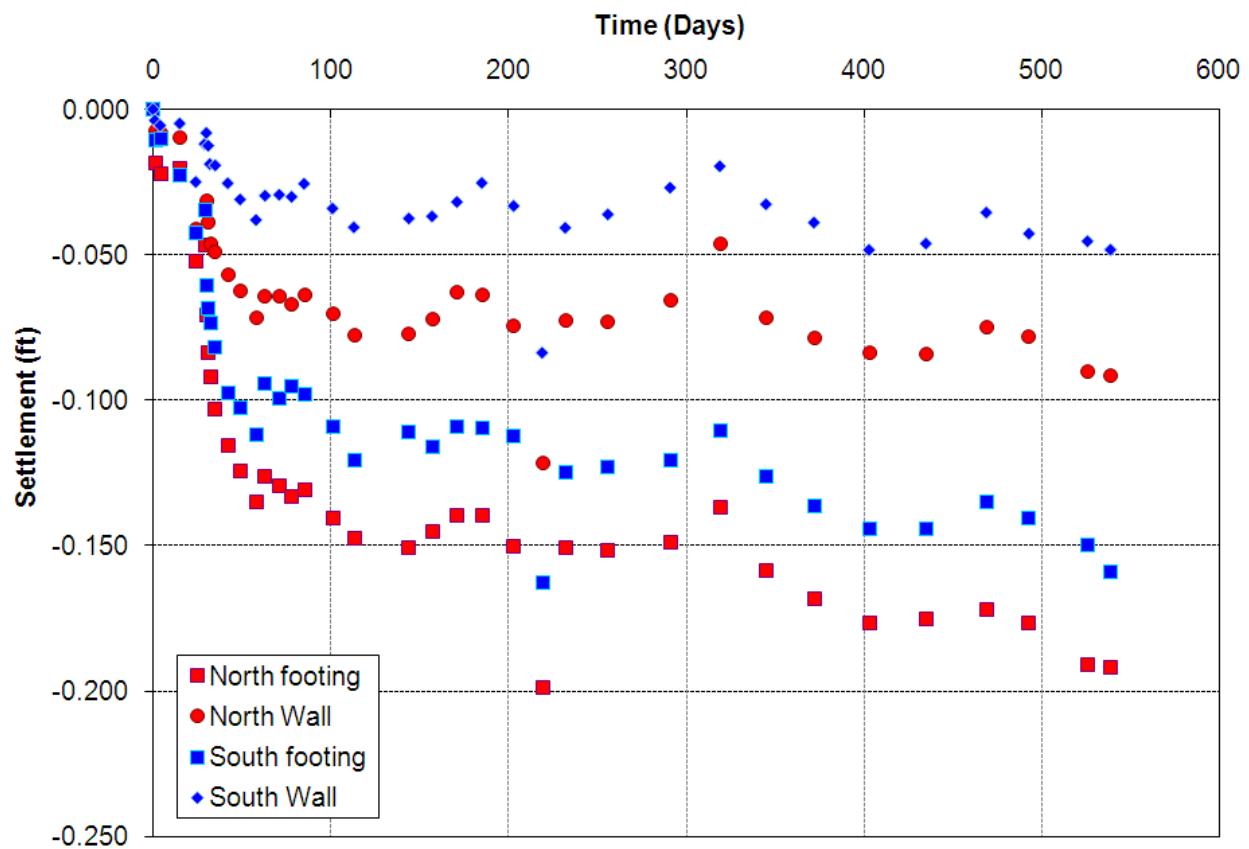
Figure 26. Tiffin River GRS-IBS settlement versus time.
