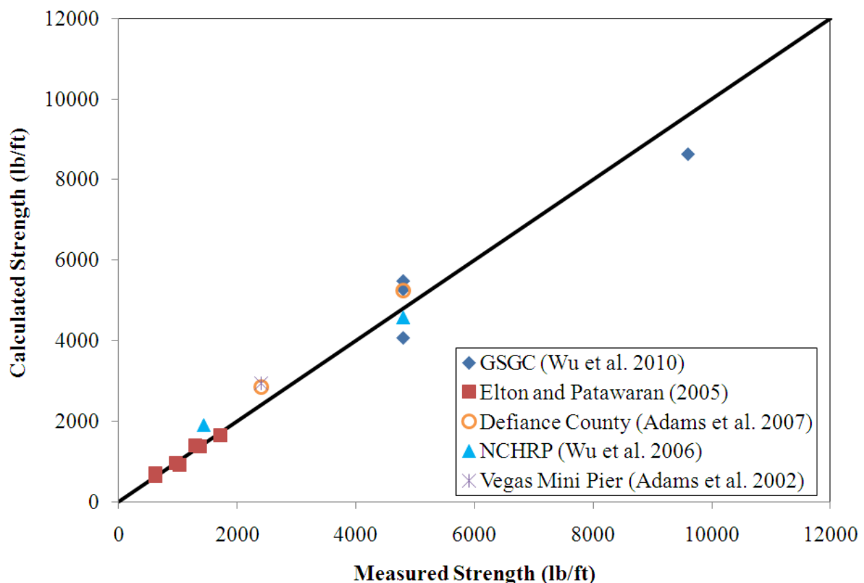
Figure 16. Predictive capability of the required reinforcement strength equation.
