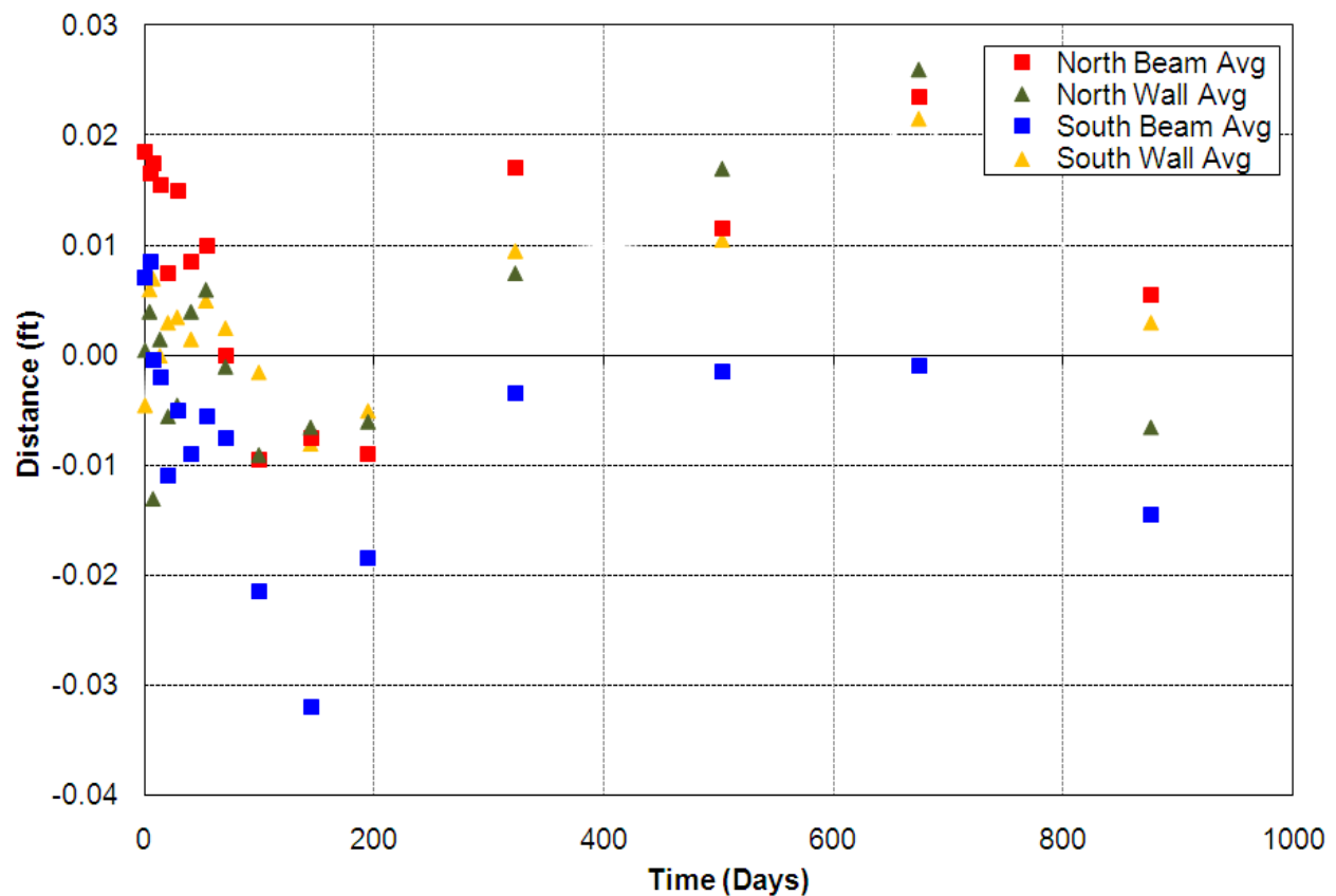
Figure 22. Huber Road GRS-IBS settlement versus time.
