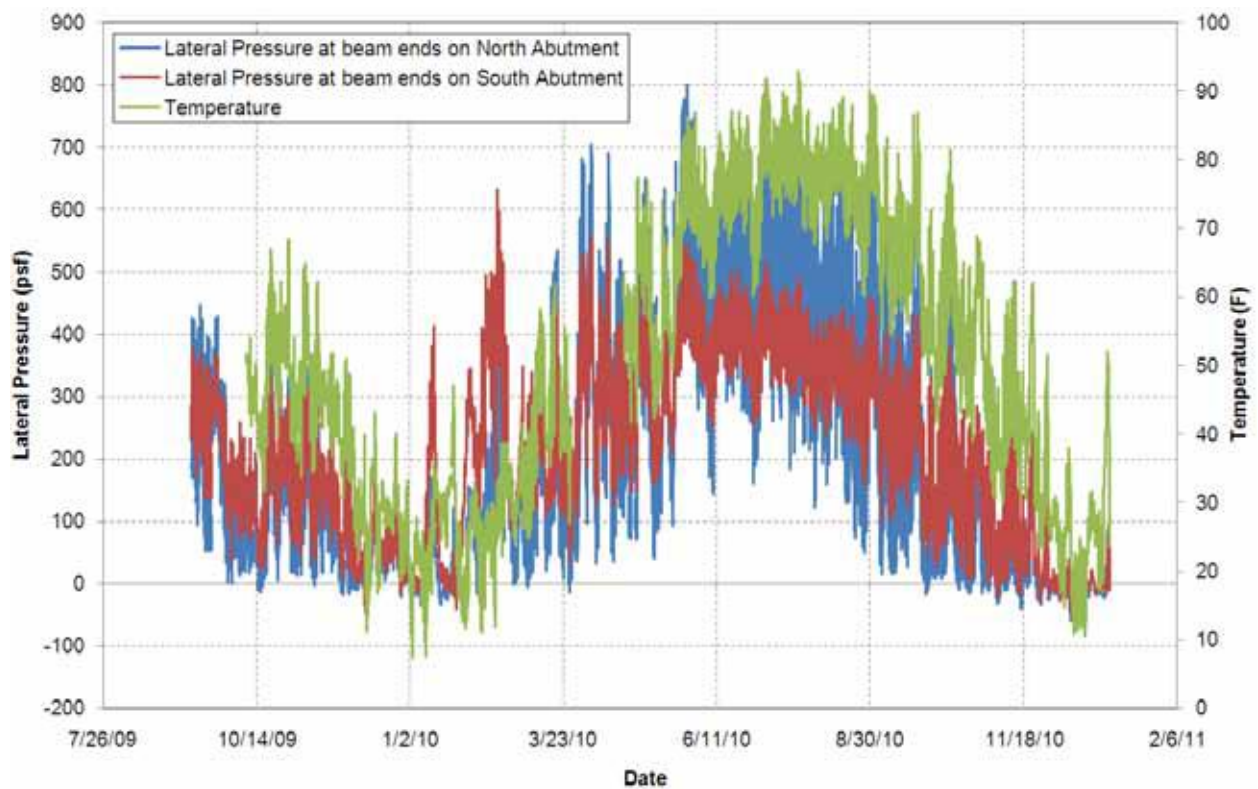
Figure 40. Average lateral pressure on back wall for Tiffin River Bridge.
