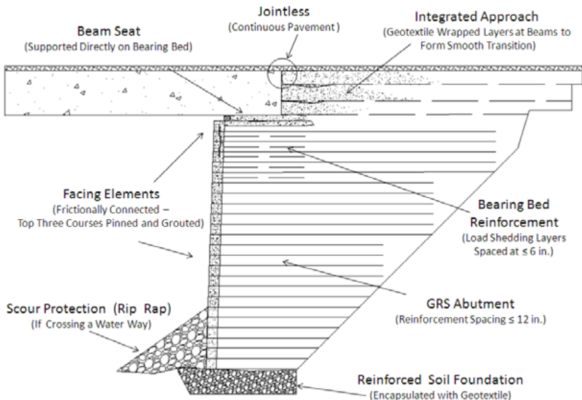
Figure 1. Typical GRS-IBS cross section.
