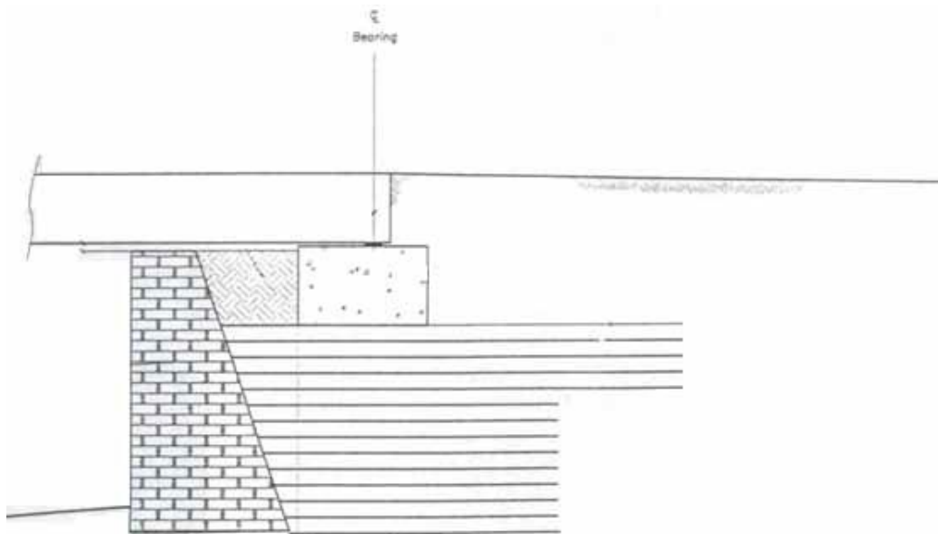
Figure 34. Cross section of GRS abutment behind historic stone abutment.
