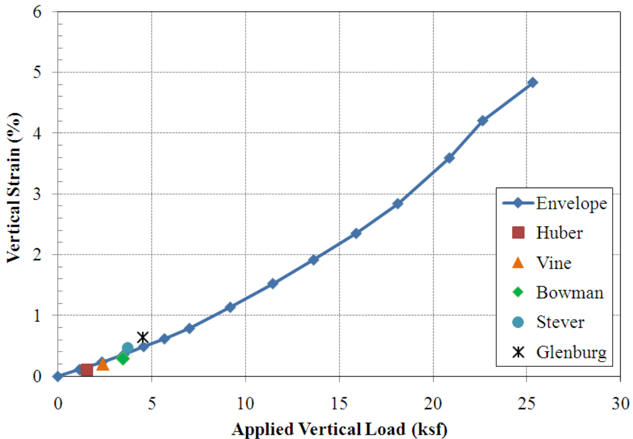
Figure 14. Deformation estimation from in-service GRS-IBS structures.
