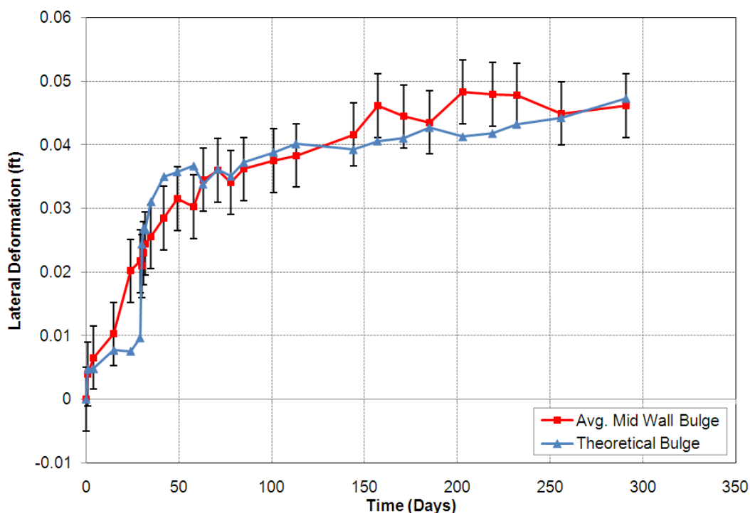
Figure 37. Measured and calculated lateral deformation on the Tiffin River Bridge GRS abutment.
