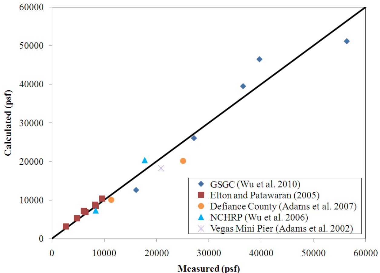
Figure 12. Predictive capability of the soil-geosynthetic composite capacity equation.
