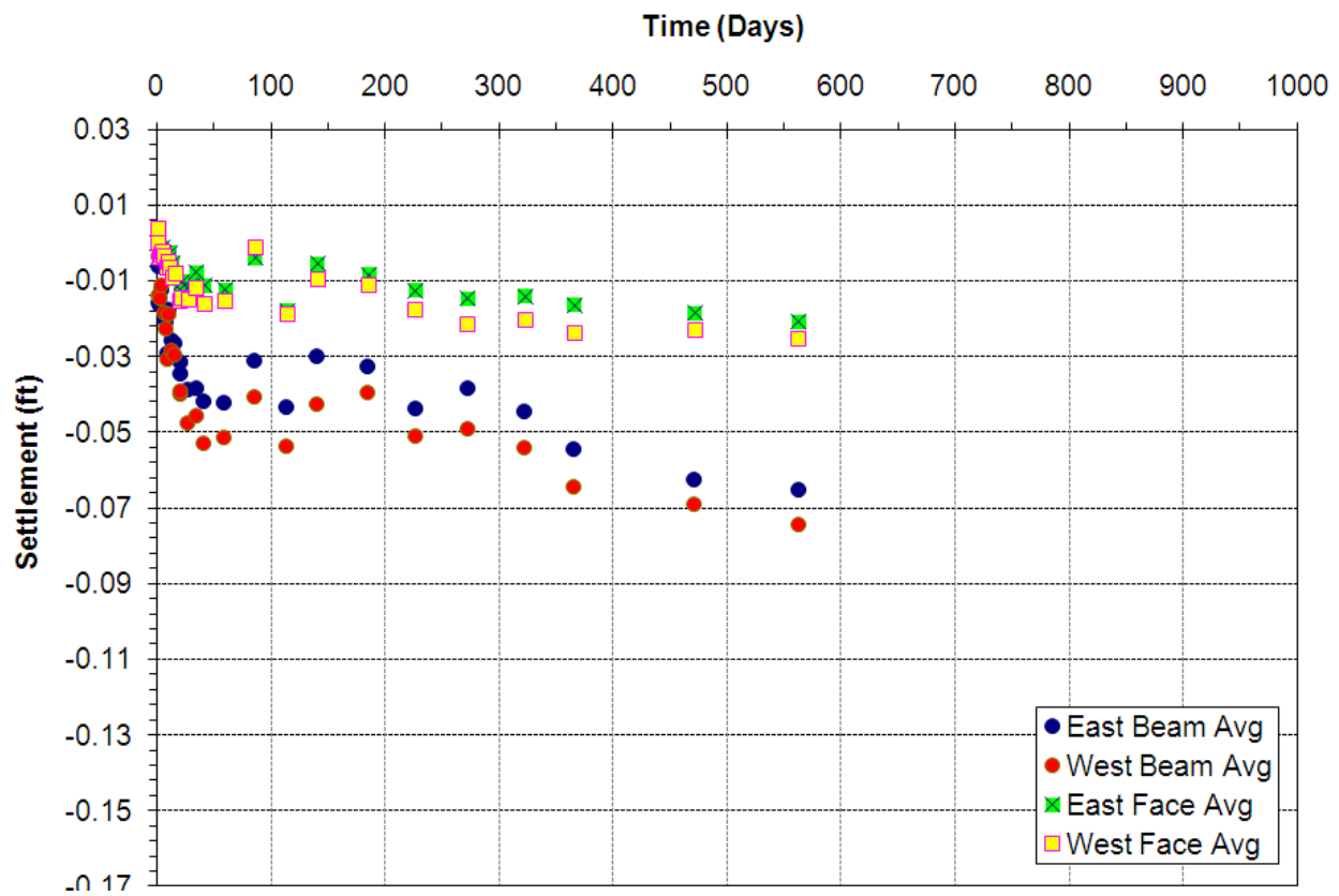
Figure 24. Bowman Road GRS-IBS settlement versus time.
