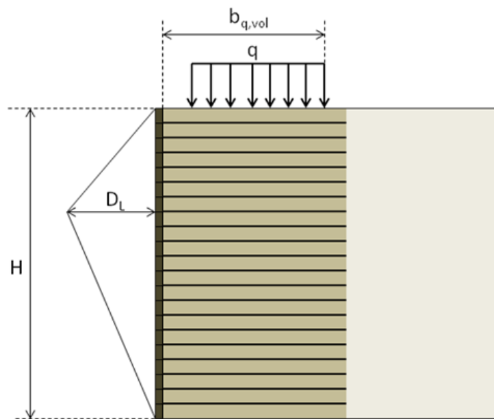
Figure 15. Lateral deformation of a GRS structure.
