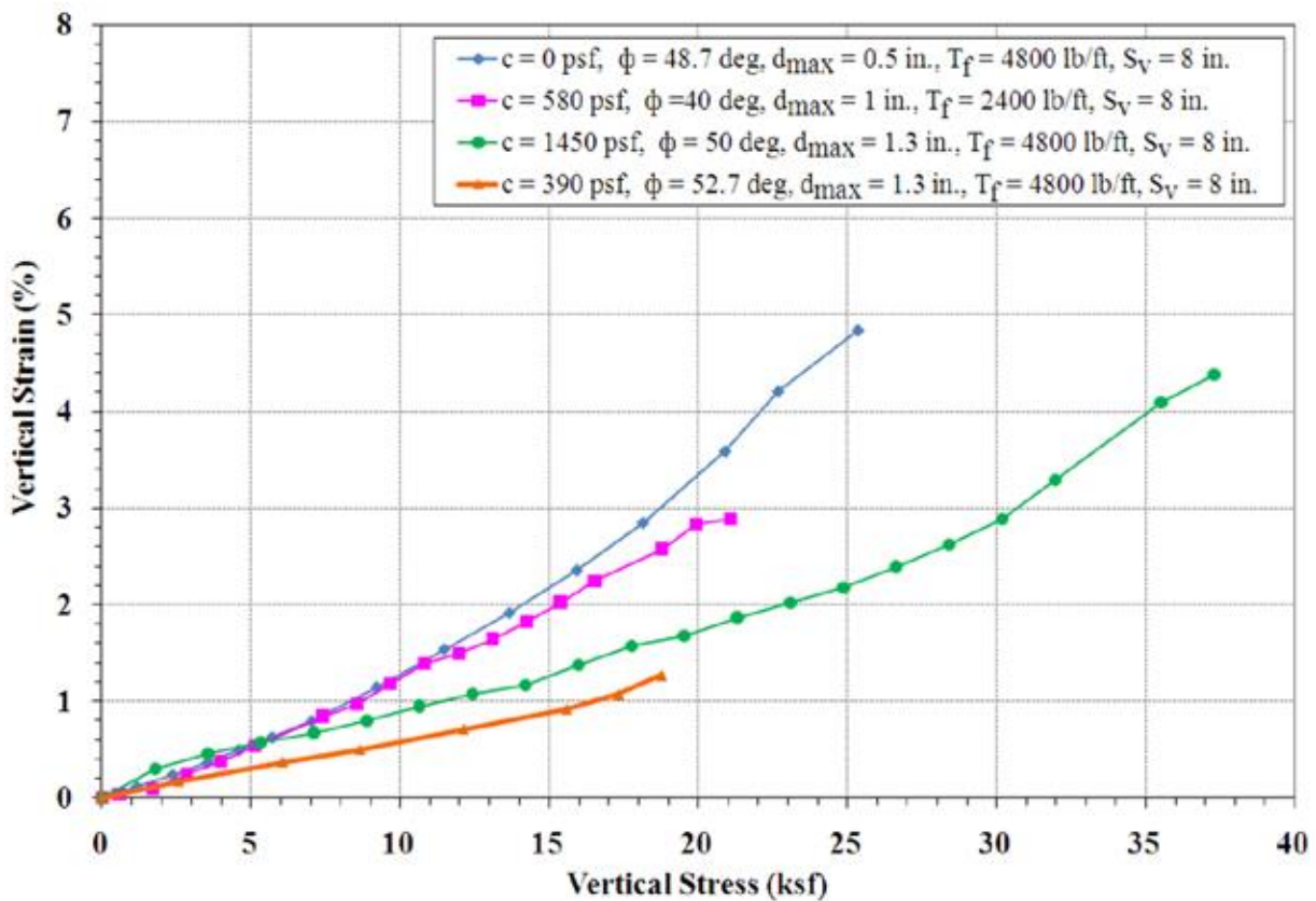
Figure 11. Graph. Performance test results for different materials.
