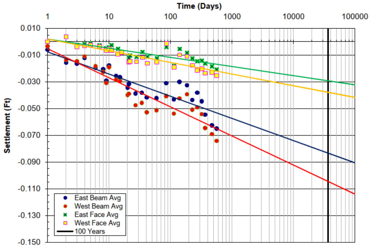
Figure 27. Settlement versus log-time to predict creep settlement for the Bowman Road Bridge at 100 years.
