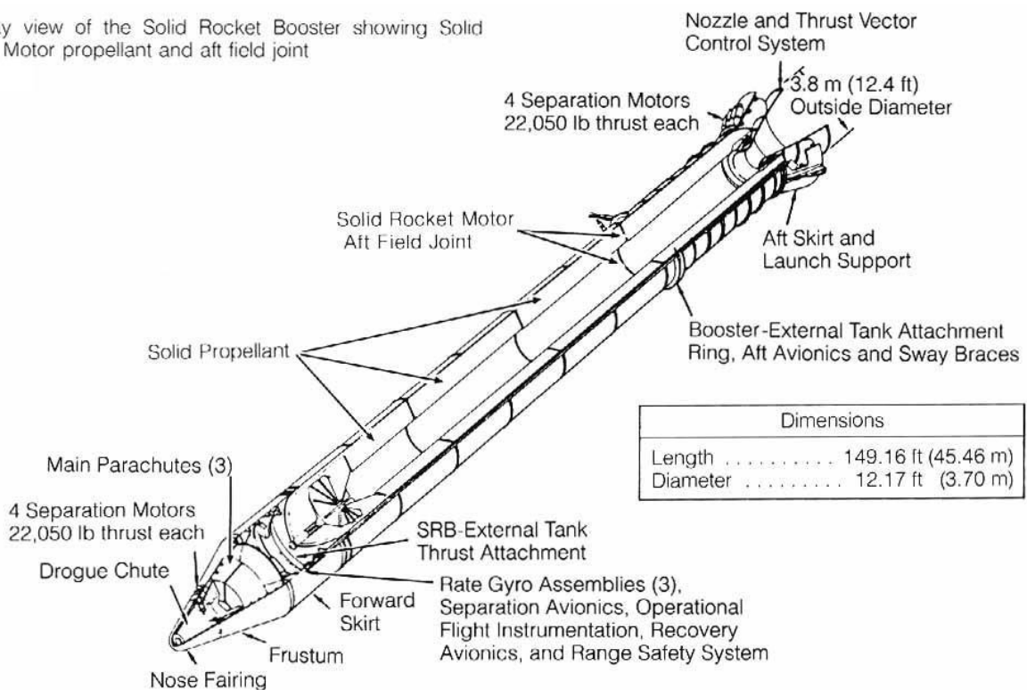
Fig. 3. Location of the Problematic Aft Field Joint
