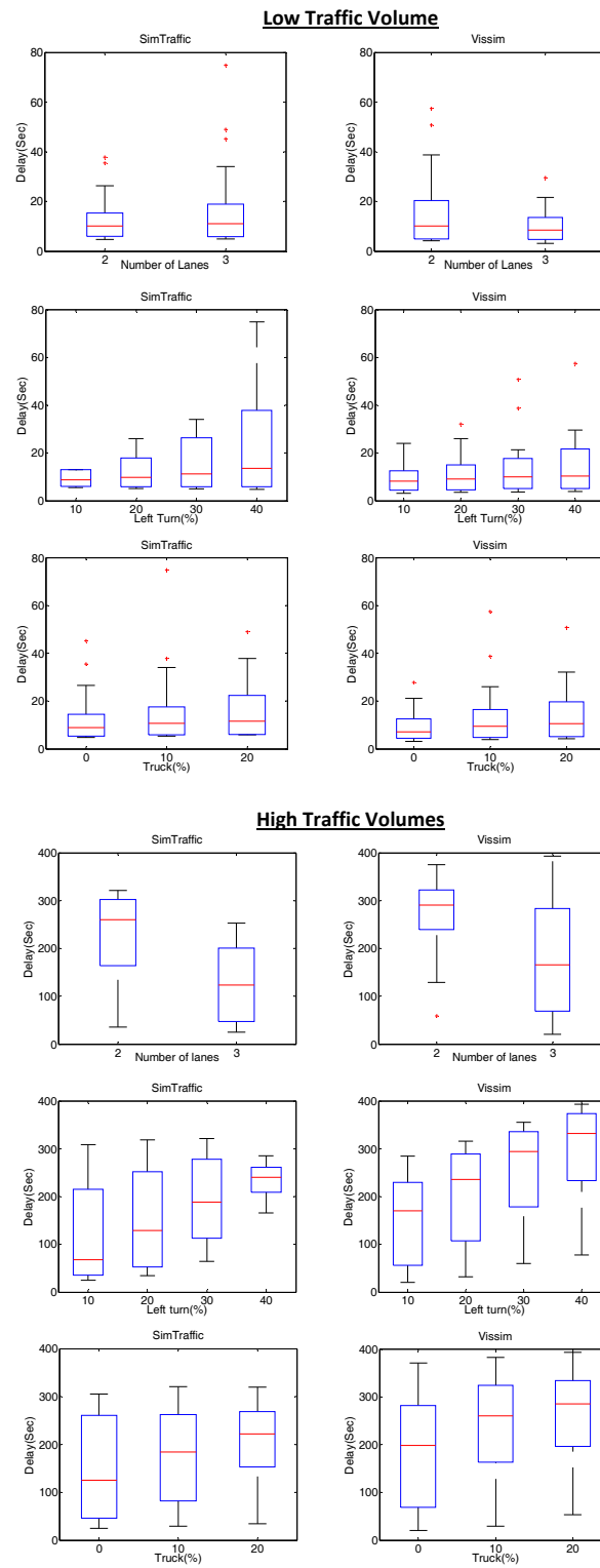
Figure 2. Average delays from SimTraffic and VISSIM against number of lanes, left turn proportion, and truck proportion at (a) low and (b) high traffic volumes
