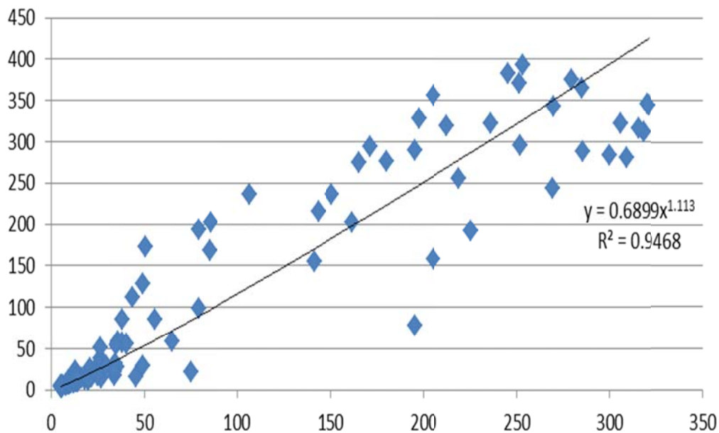
Figure 3. Correlation between SimTraffic and VISSIM
