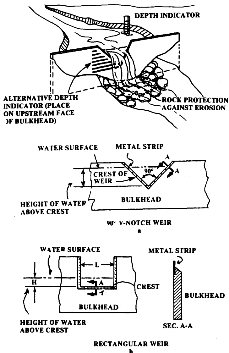
Figure 6.7 - Standard Weirs
