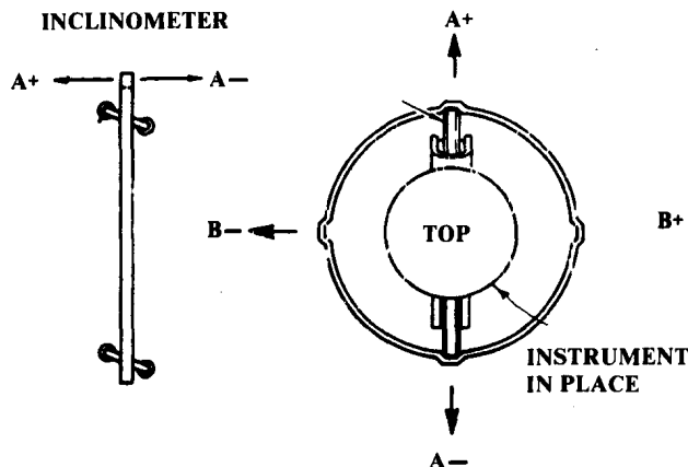
Figure 6.3c Inclinometer and Casing
