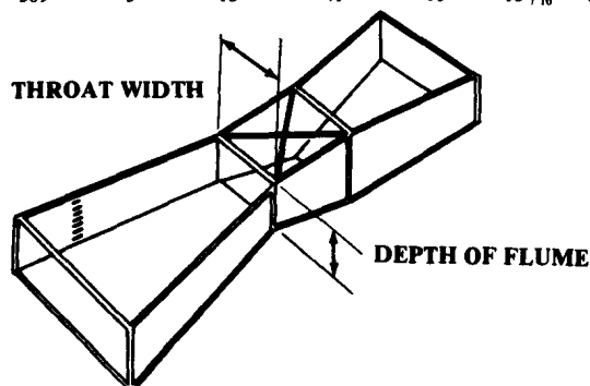
Figure 6.8 Parshall Flume
