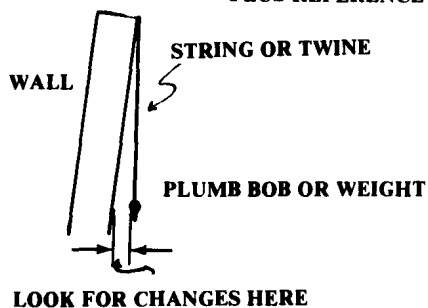
(c) PLUMB BOB
