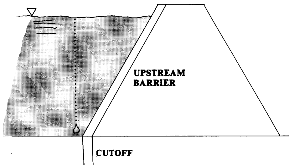
Figure 2.2 Embankment Dam
