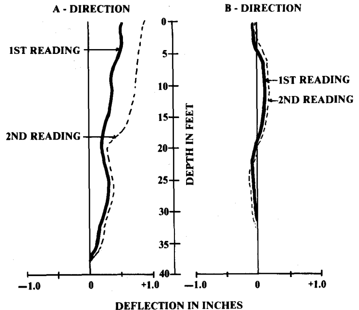
Figure 6.3b - Plot of Inclinometer Readings
