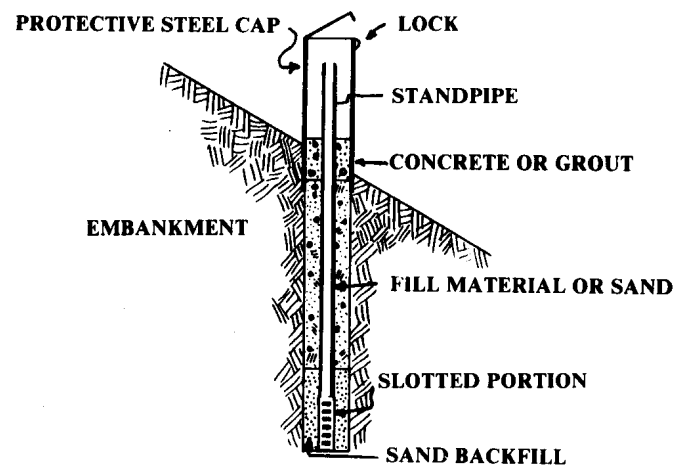
Figure 6.6 - Typical Observation Well Installation
