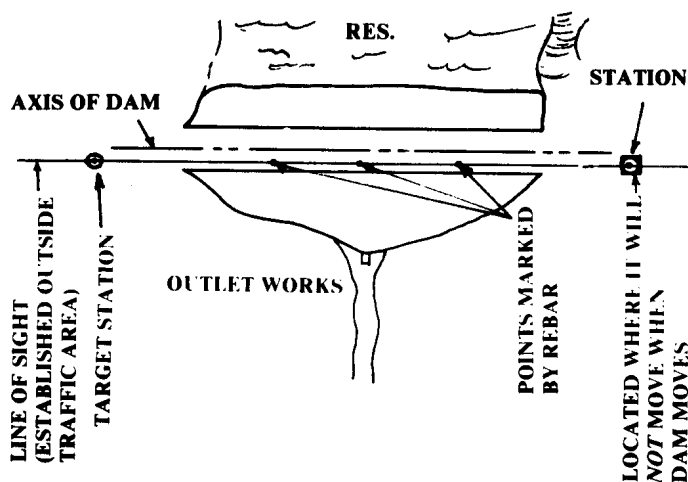
Figure 6.1b - Plan of Alignment System
