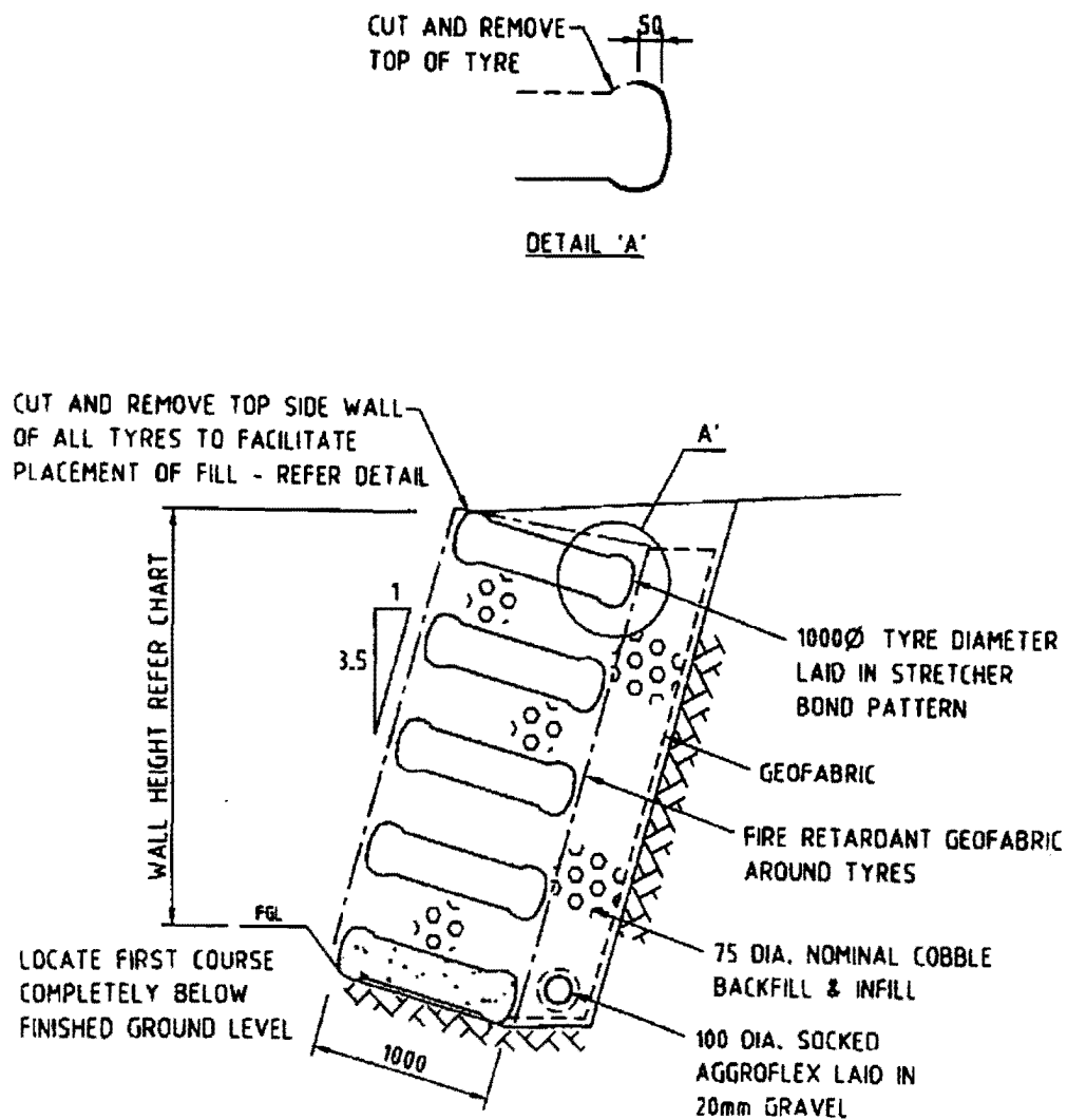
Figure 2.3. Typical Wall Section (9)
