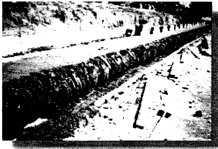
Figure 2.21: Encapsulation of Tire Bales in Concrete (12)
